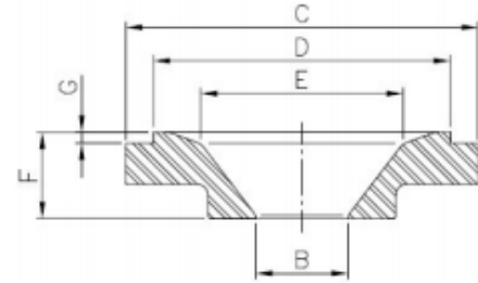
Tank Bottom Flange
